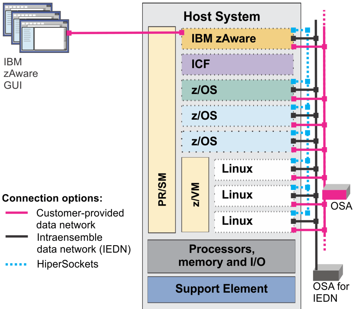
Figure 15. Supported network connection options for the IBM zAware environment
