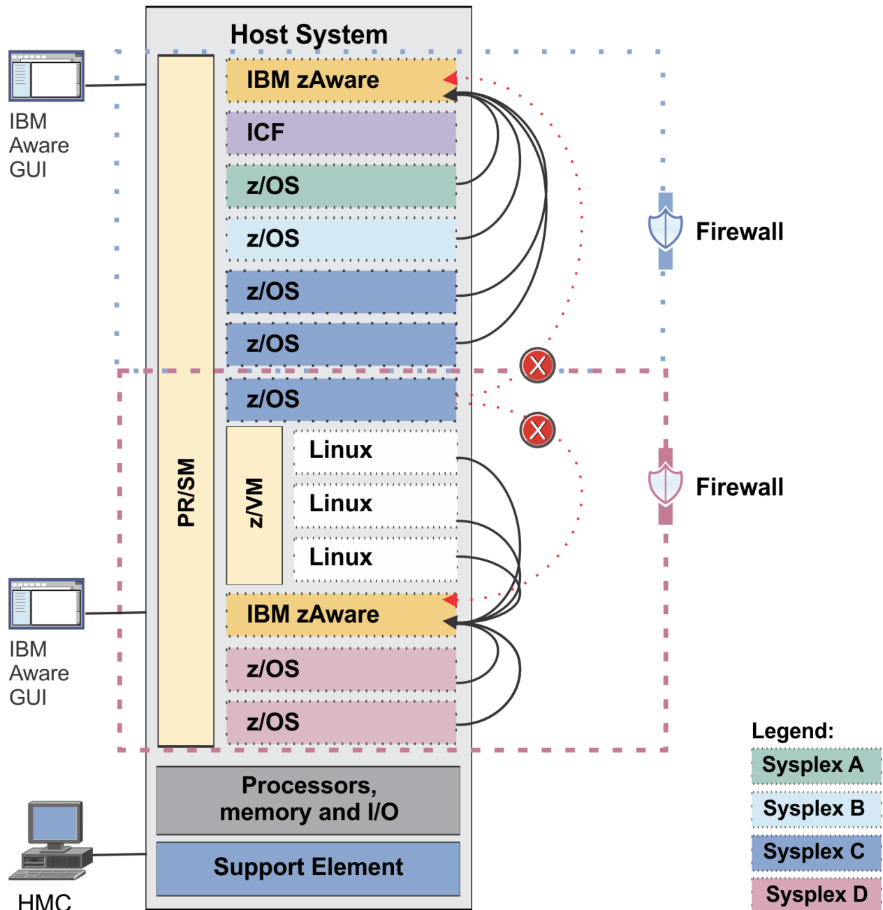
Figure 13. Two IBM zAware partitions in one host system with multiple firewalls
