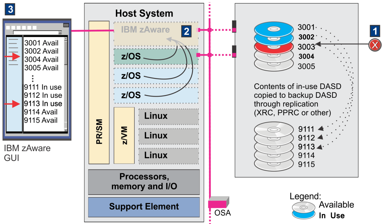
Figure 20. What happens when an in-use storage device becomes unavailable
