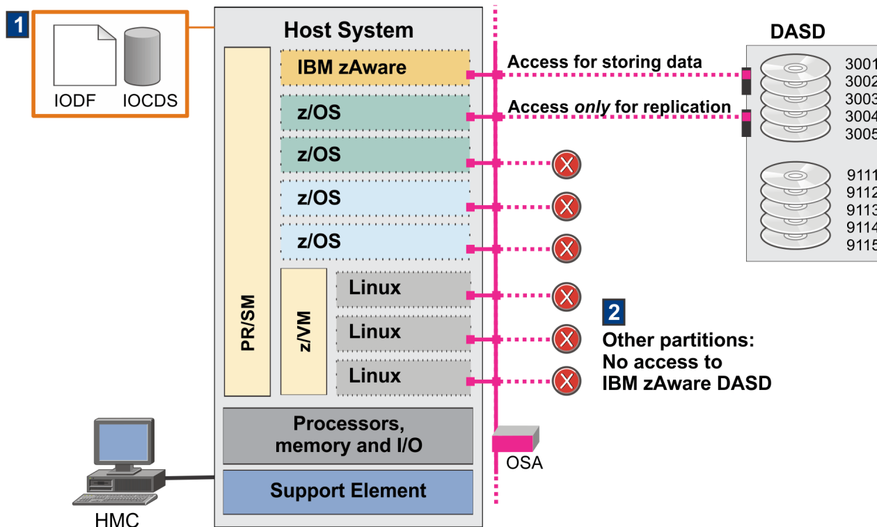
Figure 18. DASD configuration for normal operations, with access for one z/OS partition only to back up IBM zAware data
