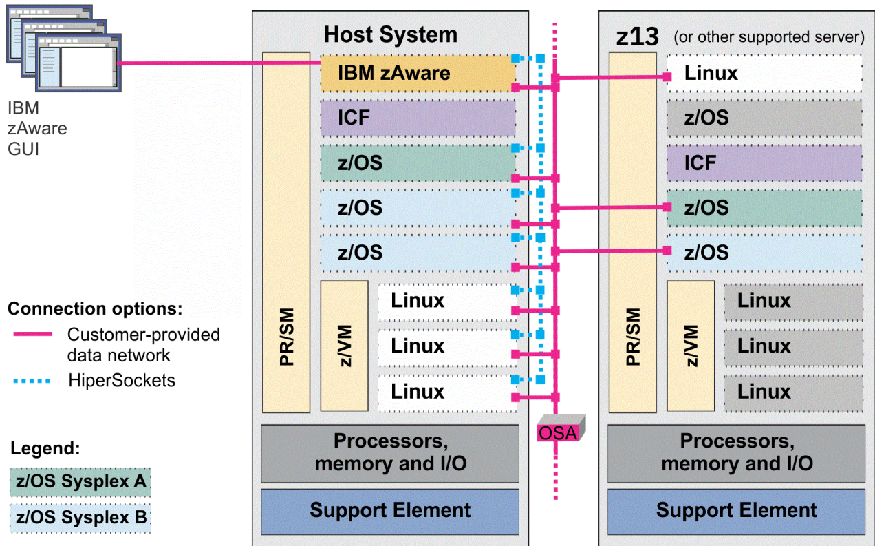
Figure 16. Network connections for an IBM zAware partition supporting clients in the host system and one z13 CPC
