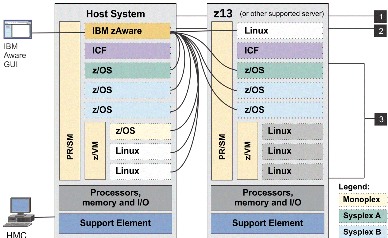
Figure 4. An IBM zAware partition supporting clients in the host system and in one z13
